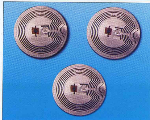
Figure 1. A typical RFID tag for 13.56 MHz. The chip is too small to see, but you can make out the fine copper loop pattern that is the antenna. Courtesy of Texas Instruments.
